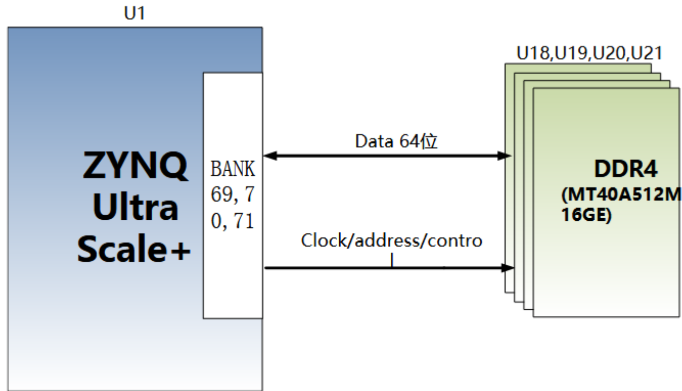
Figure 2-3-2: PL DDR4 DRAM block diagram
